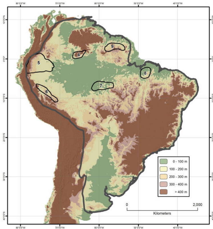
FIGURE 2 Elevation of Haffer (1969) proposed bird Pleistocene refuges on an elevation map. Numbers correspond to Haffer's original numbering of Pleistocene refuges: Imerí Refuge (4), Napo Refuge (5), East Peruvian Refuge (6), Madeira-Tapajós Refuge (7), Belén Refuge (8), and Guianan Refuge (9). Map by J. Zebrowski.
