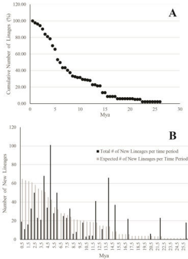
FIGURE 3 (A) Cumulative frequency of crown species development in the Amazon across a unbiased sampling of taxa from Rull (2008). The figure shows periods of stasis where no new lineages appeared punctuated by jumps corresponding with speciation pulses. These jumps are consistent with the predictions of the BDH. (B) Histogram of new lineages appearing in the last 26 My and the expected number of new lineages under the assumption of a uniform speciation rate based on the number of existing lineages. Data from Rull (2008).
